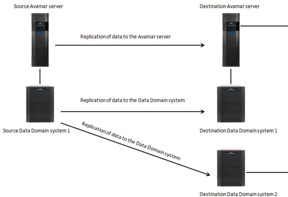
Figure 5. Data Domain system replication one to many configuration
